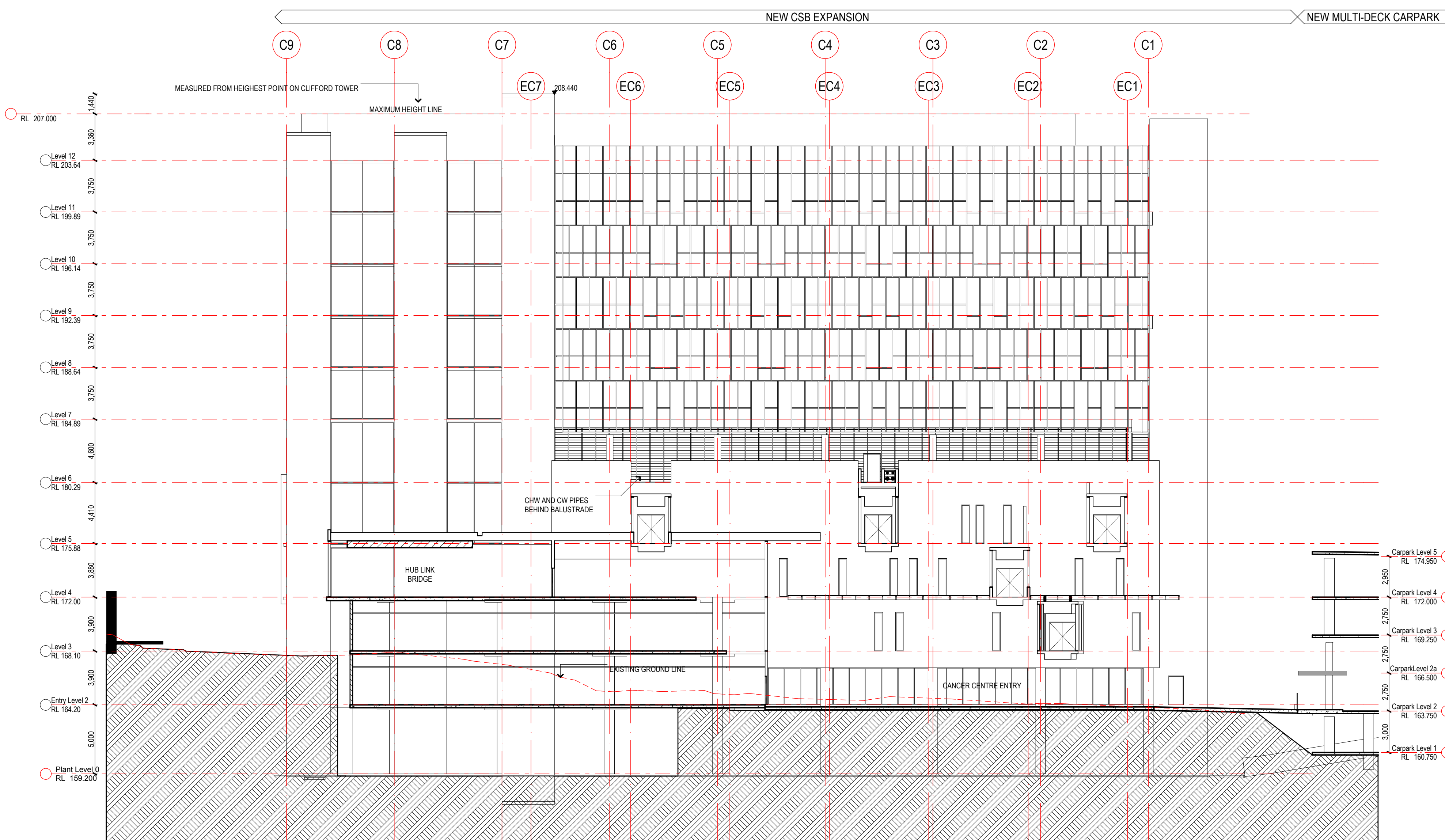
D-D SECTION D SCALE 1:200
