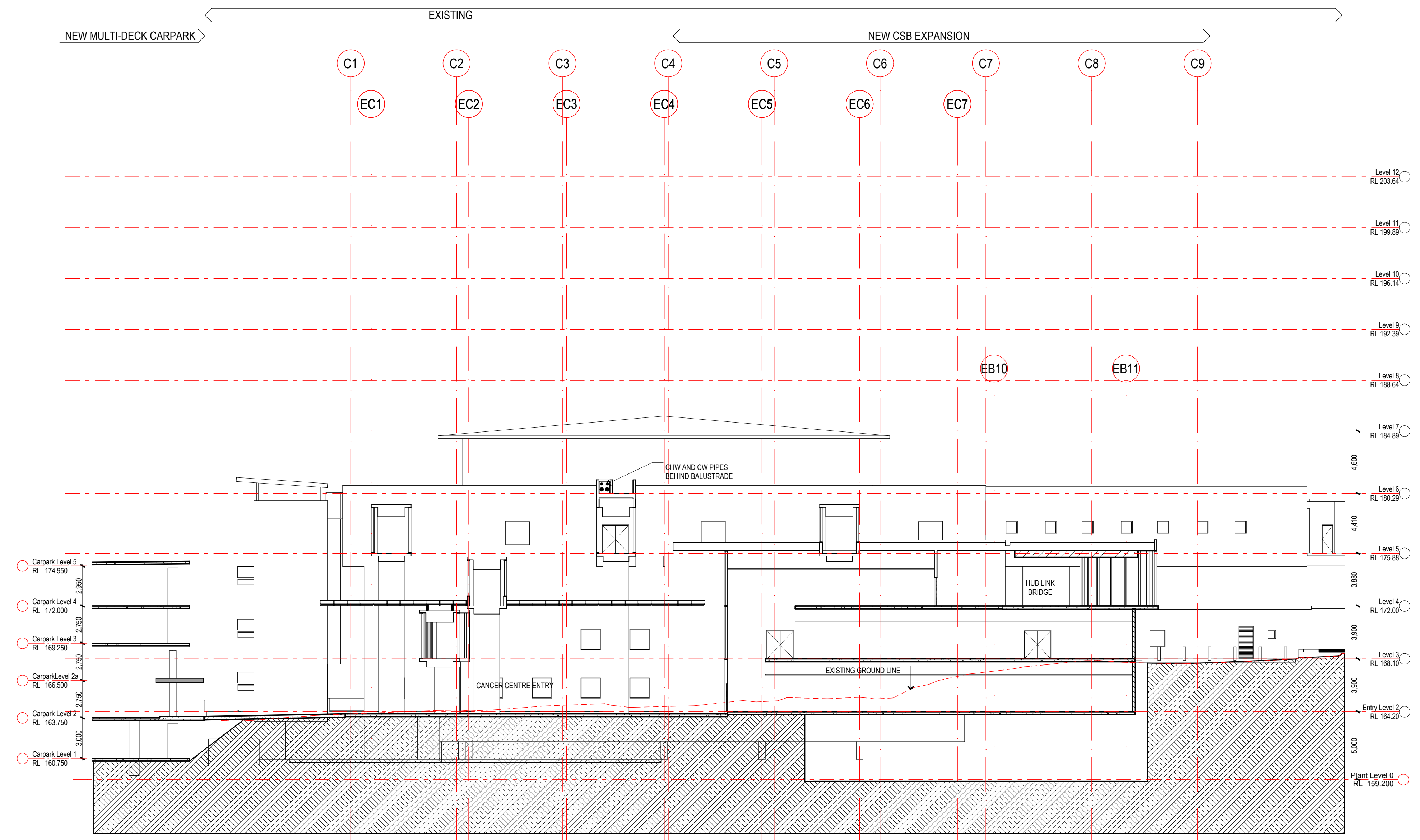
C-C SECTION C SCALE 1:200
